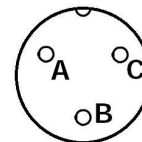
View of female connector: MS 3106A-10SL-3S (deliver with sensor without cable)
