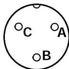
View of male connector: MS 3102A-10SL-3P (assembled on sensor)
