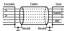
M12 8-pin
