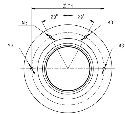
AMM80 - Mounting requirements
